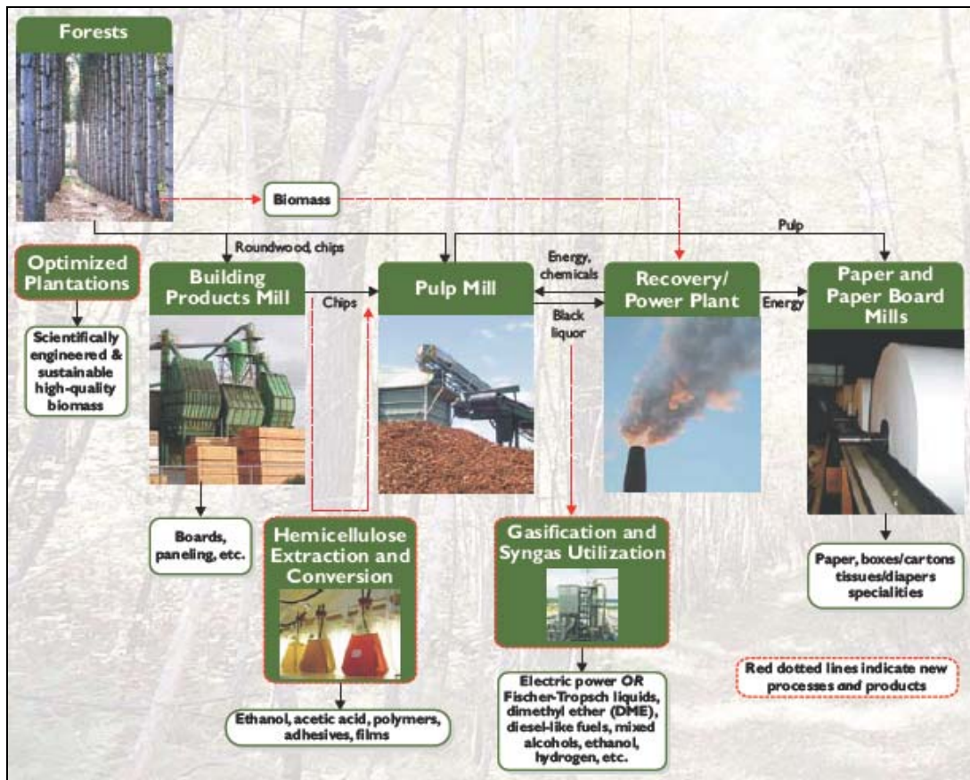
Figure 6. Integrated Biorefinery
