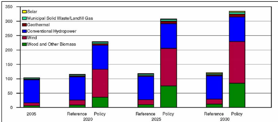
Figure 7. Renewable Generation Capacity by Energy Resource for 2005-2030 (gigawatts)
