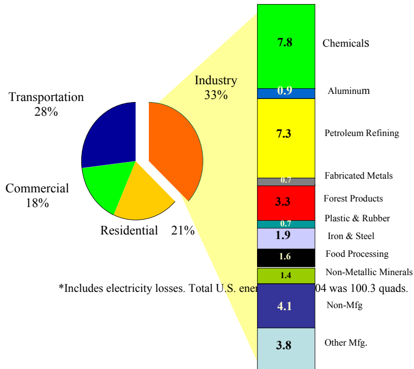
Figure 3. 2004 Energy Use in the Industrial Sector (Quadrillion Btu)*
